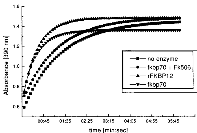
Fig. 4. Peptidyl-prolyl isomerase (PPIase) activity of recombinant FKBP-70 as measured by the method of Kofron et al. [32]. The data is generated by using 100 nM recombinant human FKBP-12 (rFKBP12) and 660 nM recombinant FKBP-70 (fkbp70). FK506 was used at tenfold molar excess to inhibit the enzyme reaction.
